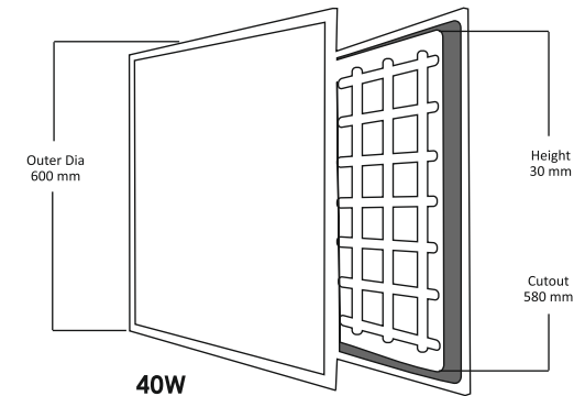
40W Product Dimension
