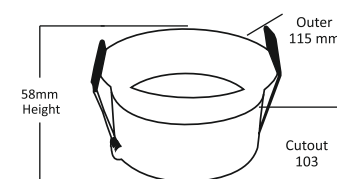
18W Product Dimension
