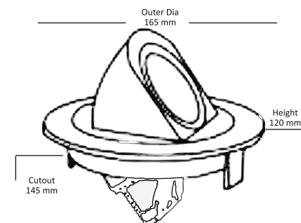
35W Product Dimension
